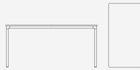
TRT1608RC. (EU) TRT6030RC. (US) Dining height table with rectangular top OH 740mm / 29" OW 1600mm / 60" OD 800mm / 30"
